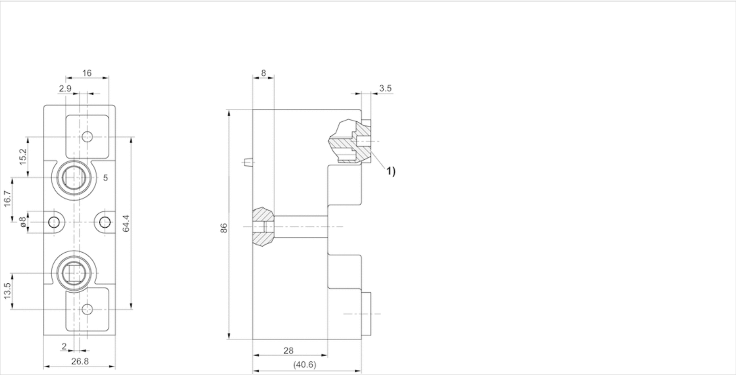
1) Mounting hole for M2.5 thread insert
