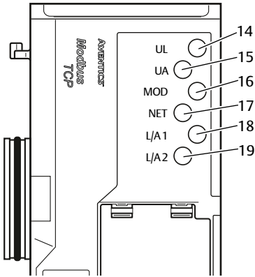
Fig. 4-7 Signification des LED
