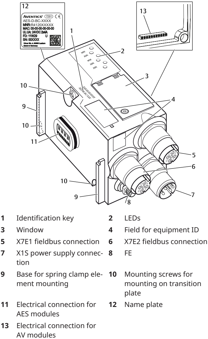
Fig. 4-1 Product overview bus coupler
