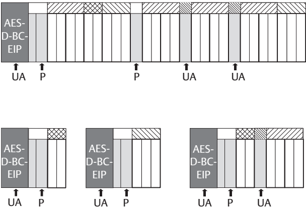
Fig. 12-15 Examples for impermissible configurations
