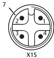
Fig. 4-4 Power supply pin assignments
