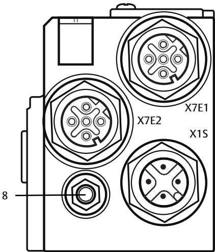
Fig. 4-6 Raccord FE
