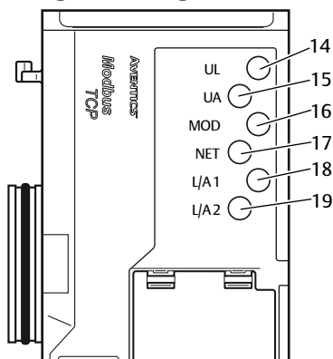
Fig. 11-1 Meaning of the diagnostic LEDs
