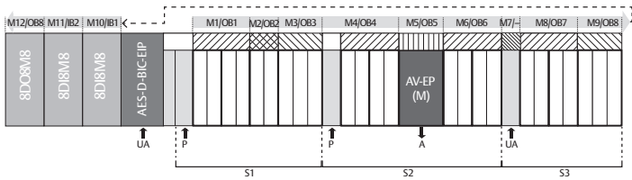
Fig. 5-1 Numbering of modules in a valve system with I/O modules
