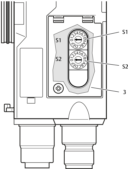
Fig. 4-8 Location of address switches S1 and S2
