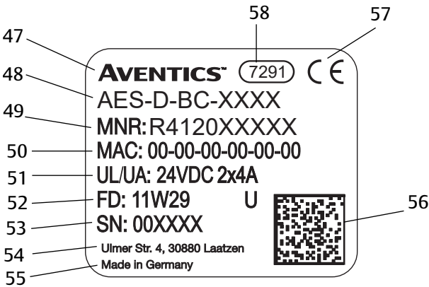
Fig. 12-12 Bus coupler rating plate
