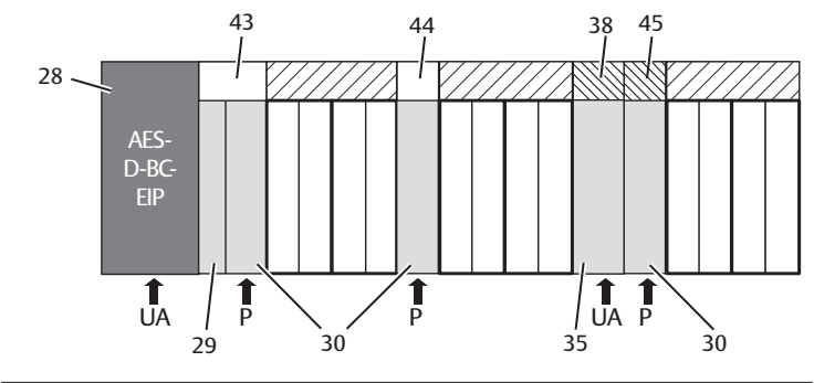
Fig. 12-10 Bridge cards and UA-OFF monitoring board
