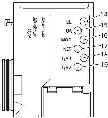
Fig. 4-7 Meaning of the LEDs
