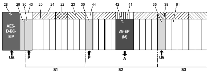
Fig. 12-13 Creating sections with two pneumatic supply plates and one electrical supply plate
