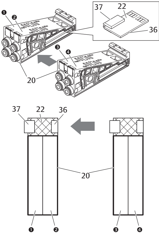
Fig. 12-7 Blocking of base plates and valve driver boards
