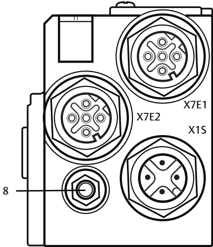
Fig. 4-6 FE connection
