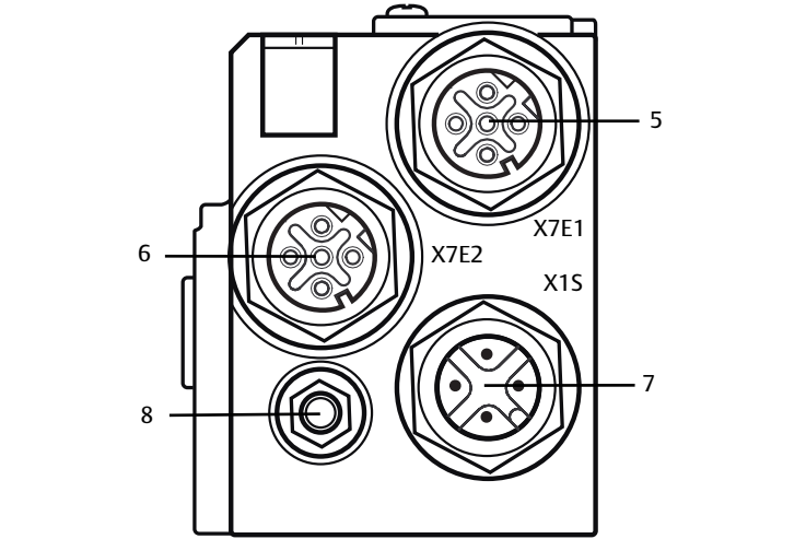
Fig. 4-2 Electrical connections of the bus coupler
