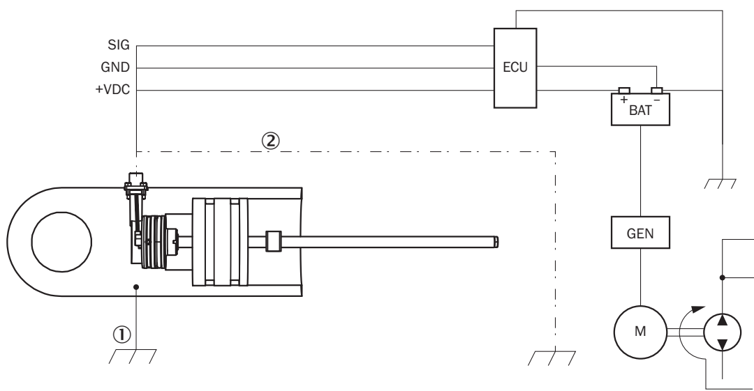
Connection diagram
