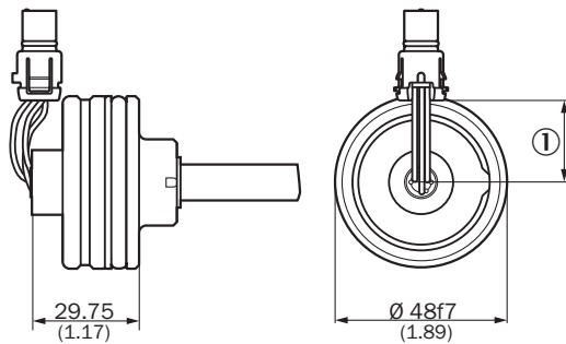
M12 male connector (analog / PWM / digital interface)
