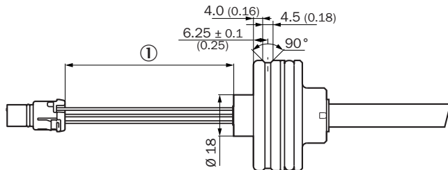
MAX48A housing
